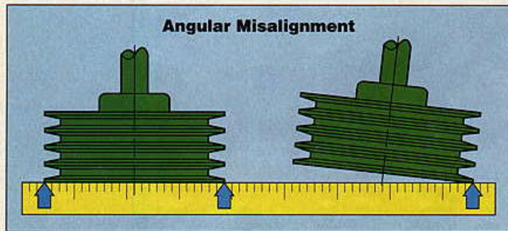
Fig. 1. Angular misalignment causes excessive belt edge cord and sidewall wear and V-belt turnover in, or escape from, sheave grooves.
